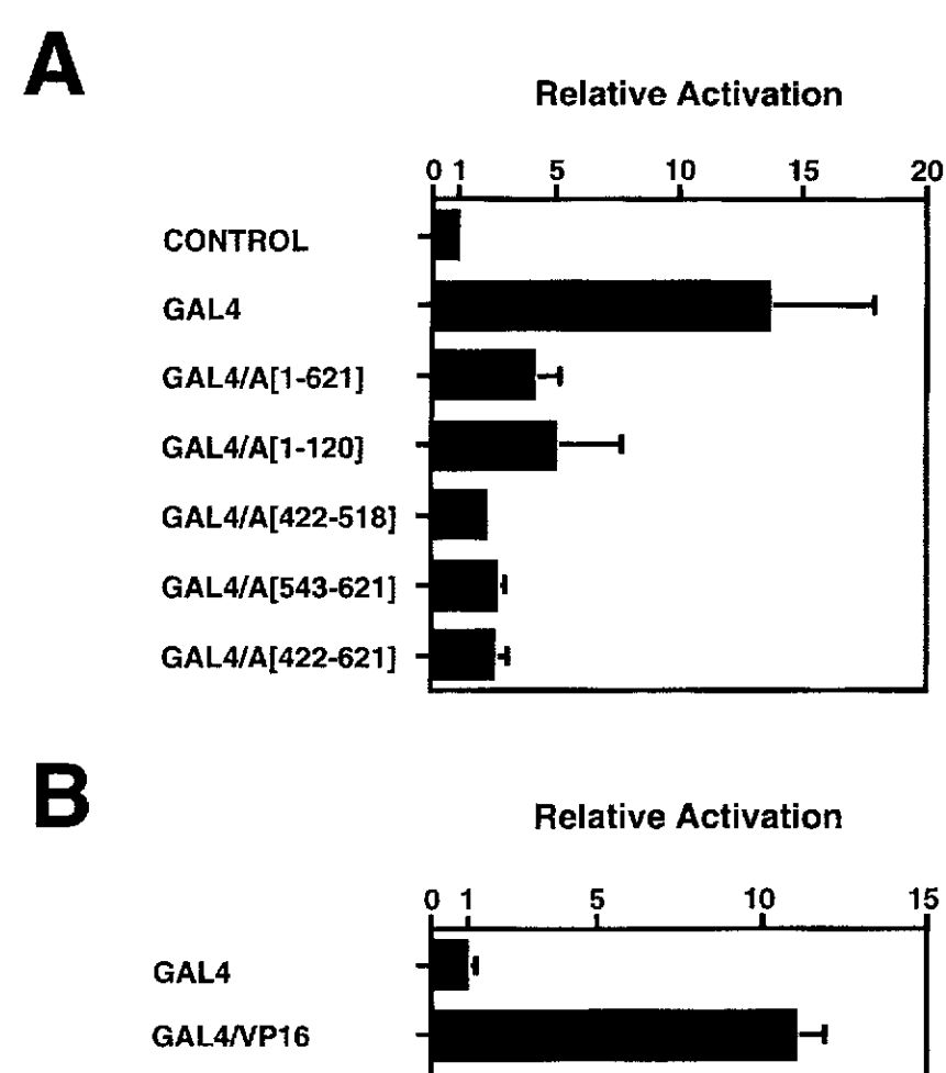
Figure 2. Expression of a GAL4-LUC reporter gene in the presence of GAL4-TnpA and GAL4-VP16 effector plasmids. A. Relative activation of the LUC reporter gene in tobacco suspension cells by expression of the chimeric GAL4/TnpA genes shown in Fig. 1. The activity of the test plasmid was measured and normalized to an internal CAT control as described in Materials and methods. Relative activation represents the ratio of normalized LUC activity obtained in the presence of a GAL4- or a GAL4/TnpA effector plasmid to that observed with an effector plasmid carrying an antisense GAL4/VP16 construct. The LUC reporter plasmid contains GAL4 DNA binding sites and a minimal CaMV 35 S promoter (Fig. 1B). B. Activation of the LUC reporter gene by the chimeric GAL4/VP16 construct shown in Fig. 1. Relative activation is the ratio of normalized LUC activity observed in the presence of the GAL4/VP16 fusion to that observed with GAL4-binding domain alone.
