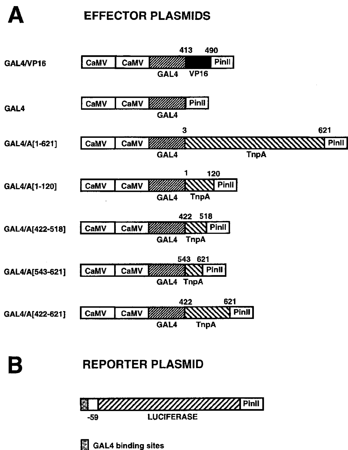
Figure 1. Schematic representation of GAL4 fusion genes and the luciferase reporter gene. A. Effector plasmids are those that encode a trans -acting activator or repressor of the luciferase reporter gene. Each construct contains the yeast GAL4 DNA binding domain either alone or translationally fused to the following: VP16, the strong activation domain of the herpes simplex virus VP16 (amino acids [a.a.] 413 to 490); A[3–621], full-length TnpA (a.a. 3 to 621); A[1–120], N-terminus of TnpA (a.a. 1–120); A[422–518], the protein dimerization domain of TnpA (a.a. 422 to 518); A[543–621], C-terminus of TnpA (a.a. 543 to 621); A[422–621], the dimerization domain and C-terminus of TnpA (a.a. 422 to 621). PinII, potato proteinase inhibitor II terminator; CaMV, cauliflower mosaic virus 35S promoter. B. The reporter plasmid contains 5 GAL4 DNA-binding sites upstream from a truncated CaMV promoter (bp –59 to +2) and the firefly luciferase gene.
