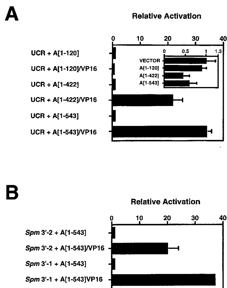
Figure 4. Activation of the Spm promoter by TnpA/VP16 fusion proteins in tobacco cells. A. Relative activation of UCR-LUC reporter gene expression (Fig. 3B) by the chimeric TnpA/VP16 fusion proteins shown in Fig. 3A. Controls were plasmids carrying the corresponding TnpA gene or gene fragments lacking the VP16 activation domain. LUC activity was measured and normalized as described in Materials and methods. Relative activation is the ratio of normalized LUC activity observed in the presence of the effector plasmid expressing the TnpA/VP16 to that observed with an effector plasmid expressing only the corresponding TnpA gene or gene fragment. The insert shows the corresponding relative activation values for the TnpA gene fragments relative to the bluescript pKS(+) vector control. B. Relative activation of two different Spm 3'-LUC reporter gene expressions (Fig. 3B) by chimeric TnpA[1-543]/VP16. The Spm 3' end contains 15 TnpA-binding sites.
