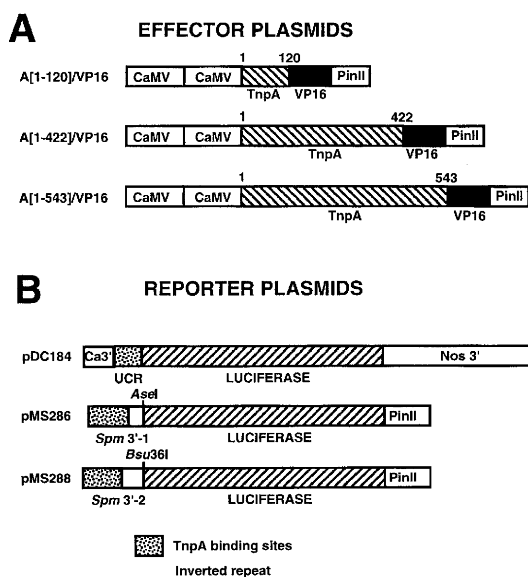
Figure 3. Schematic representation of chimeric TnpA-VP16 and Spm promoter-luciferase reporter genes. A. Effector plasmids contain translational fusions of the following TnpA domains to the herpes simplex VP16 activation domain (a.a. 413 to 490): A[1-120], N-terminus of TnpA (a.a. 1 to 120); A[1-422], N-terminus and DNA-binding domain of TnpA (a.a. 1 to 422); A[1-543], N-terminus, DNA-binding and protein dimerization domains of TnpA (a.a. 1 to 543). PinII, potato proteinase inhibitor II terminator; CaMV, cauliflower mosaic virus 35S promoter. B. The firefly LUC gene in the reporter plasmids is expressed from either the UCR promoter sequence of the Spm element, which contains 9 TnpA-binding sites, [17], or 1 of 2 different fragments of the Spm 3'-end in the antisense orientation, each containing 15 TnpA binding sites [14; 8]. Nos 3', nopaline synthase terminator. Ca3', CaMV 35S terminator; PinII, potato proteinase inhibitor II terminator.
