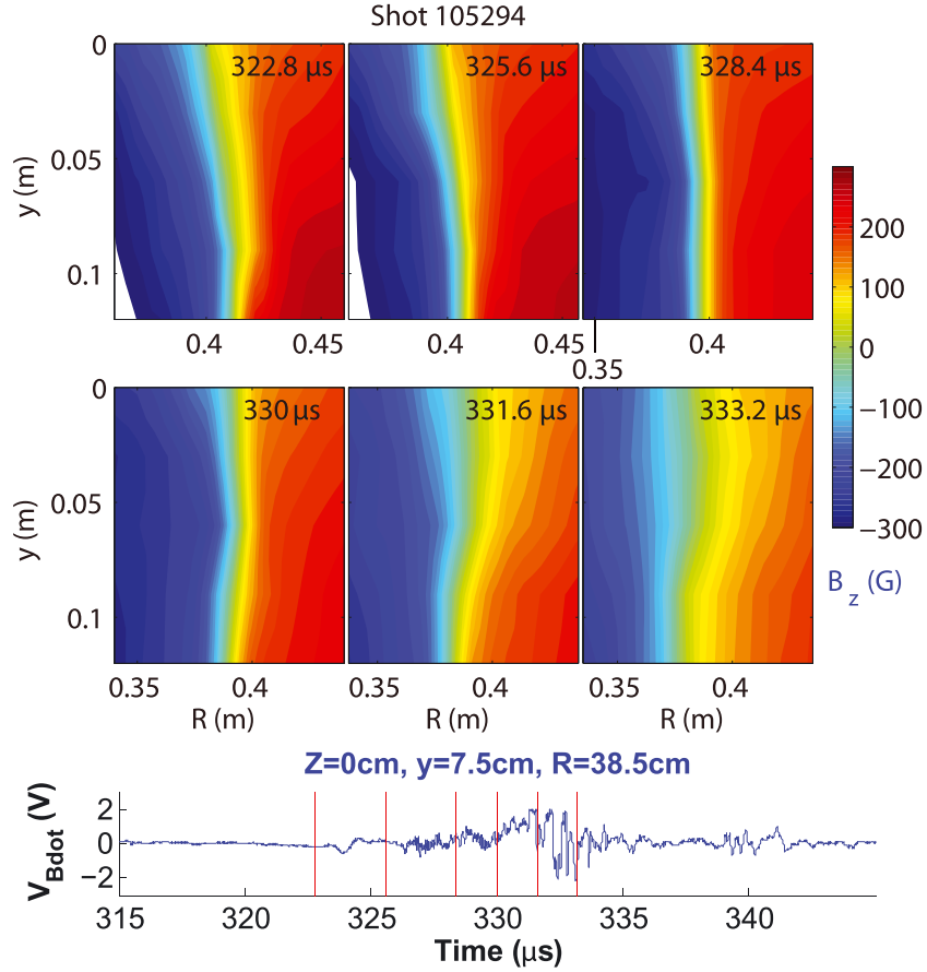
Figure 4. Out-of-plane view of current density increase and subsequent disruption. Magnetic field B_z is plotted at six times as a function of R and y for an 8.5 mTorr deuterium discharge. The top row shows the buildup phase with time increasing to the right, while the second row shows the disruption. Note that the disruption spreads from top to bottom in the electron flow (+ y ) direction. Also shown in the bottom panel of the figure is a plot of magnetic fluctuations measured at Z=0 cm, y=7.5 cm, and R=38.5 cm with the six times for the upper plots indicated by vertical red lines.
