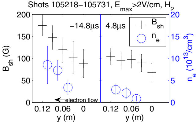
Figure 3. Probe measurements of out-of-plane gradients before a current layer disruption and prior to flux rope formation (left) and after the disruption (right). Black crosses represent the upstream magnetic field obtained from fitting the experimental data to a Harris profile [14] in the inflow region at Z=0 . Blue circles show density measured at the current sheet center at Z=2.6 cm. Data are averaged over 101 hydrogen discharges at 10.8 mTorr with a peak inductive electric field of at least 2 V/cm at y=6 cm. The time indicated in the upper portion of each panel is with respect to the disruption time. In the pull phase initial condition, there are strong gradients in both quantities in the out-of-plane electron flow ( +y ) direction. Following the disruption, the original magnetic field gradient has relaxed, and density is lower.
