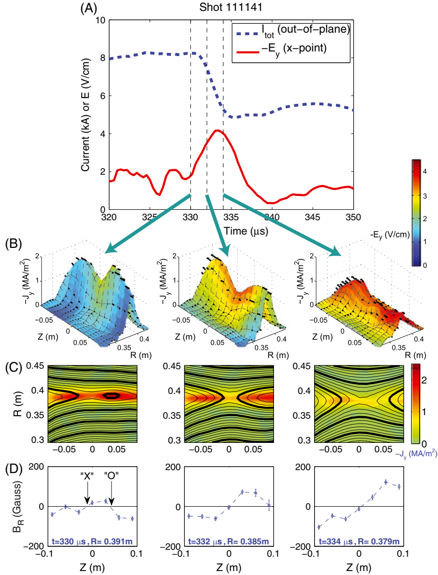
Figure 2. An example of a current layer disruption in which the electric field peaks and the current drops as a flux rope structure is ejected from the layer. (Row A) Total out-of-plane current drop and reconnection rate enhancement during a current layer disruption. Shown are the total out-of-plane current integrated over the field of view of the fine structure array (thick dashed line) and inductive electric field at the X-point (solid line) for a representative deuterium discharge at 8 mTorr. (Row B) Detailed layer profiles from the fine structure magnetic field probes for the three times indicated by the vertical dashed lines in the top panel. The height of the contours represents out-of-plane current density -J_y , obtained through differentiation of 2-D magnetic field data, the color scale inductive electric field -E_y , and the arrows in-plane current derived from the out-of-plane magnetic field. (Row C) Flux plots with current density shaded for the same three times. (Row D) B_R as a function of Z at the R location of the current sheet center as measured by the fine structure probe array. As the disruption proceeds, the layer aspect ratio decreases; at the same time, B_R increases, first near Z=0 and then at outer Z locations. X and O-points for the first time slice are marked on the figure.
