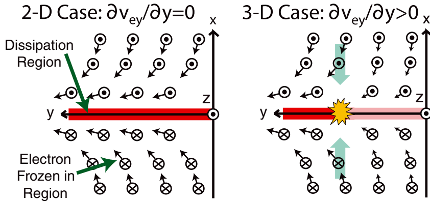
Figure 5. Diagram of the inflow region showing electron flow (arrows) convecting field line (circles) towards the dissipation region (red shaded region) in both the 2-D case with no spatial variation in the out-of-plane direction (left) and a simplified 3-D case with an out-of-plane electron flow gradient (right) associated with added y variation of B_x . B_x is not shown explicitly, but the resulting modifications to the flow pattern and current density in the 3-D case are. For example, lighter shading represents lower current density in the dissipation region due to larger \partial B_x/\partial z . The 3-D variation shown may lead to a layer disruption as described in the text.
