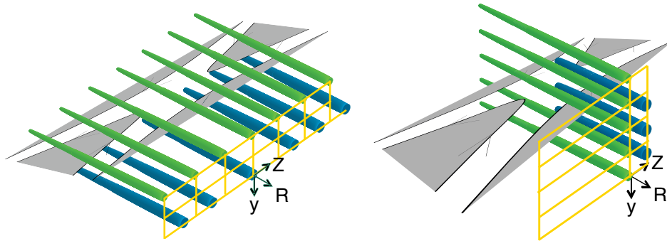
Figure 1. Probe locations in the current sheet for in-plane measurements (left) and out-of-plane measurements (right). The local coordinate system is indicated by the coordinate axes in both plots. The Cartesian coordinate y is locally oriented in the azimuthal direction of MRX. For illustration purposes, parts of the reconnection plane are shaded gray. In the left panel, seven fine structure magnetic field probes (light green), each with 35 magnetic sensors, are located in the y=0 plane on both sides of the current sheet. In the right panel, five fine structure probes, each with 50 magnetic sensors, are located at Z=0 but at various out-of-plane y positions. Probes in both setups are separated by 3 cm. Additional probes to measure density, temperature, or high frequency magnetic field fluctuations may be placed nearby in the blue positions.
