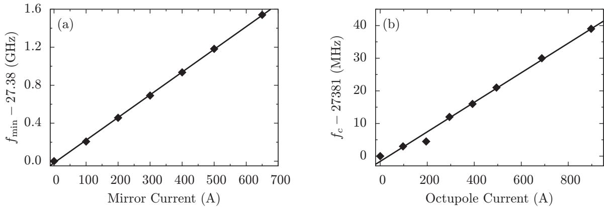
Figure 6. (a) The frequency of the minimum cyclotron resonance ( f_{\min} ) as a function of the current in mirror coil magnets. The octupole magnet is not energized during these measurements. (b) The cyclotron resonance as a function of the current in the octupole magnet. The mirror coil magnets are not energized for these measurements.
